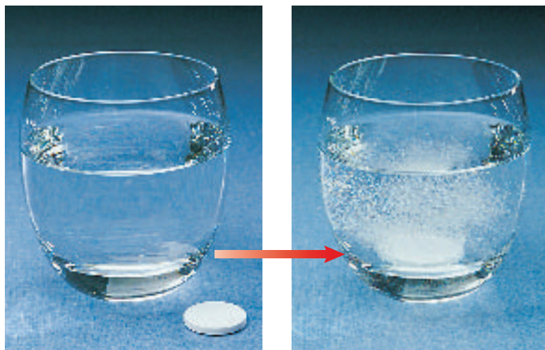
Figure 15 The bubbles of gas formed when this antacid tablet is dropped into water indicate a chemical change. The solid forming from two liquids is another sign that a chemical change has taken place.
